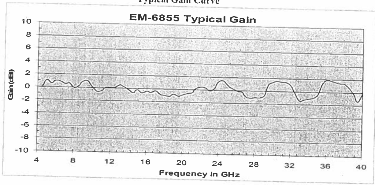
Model EM-6855 Omni-Directional Wideband Antenna Typical Gain Curve
